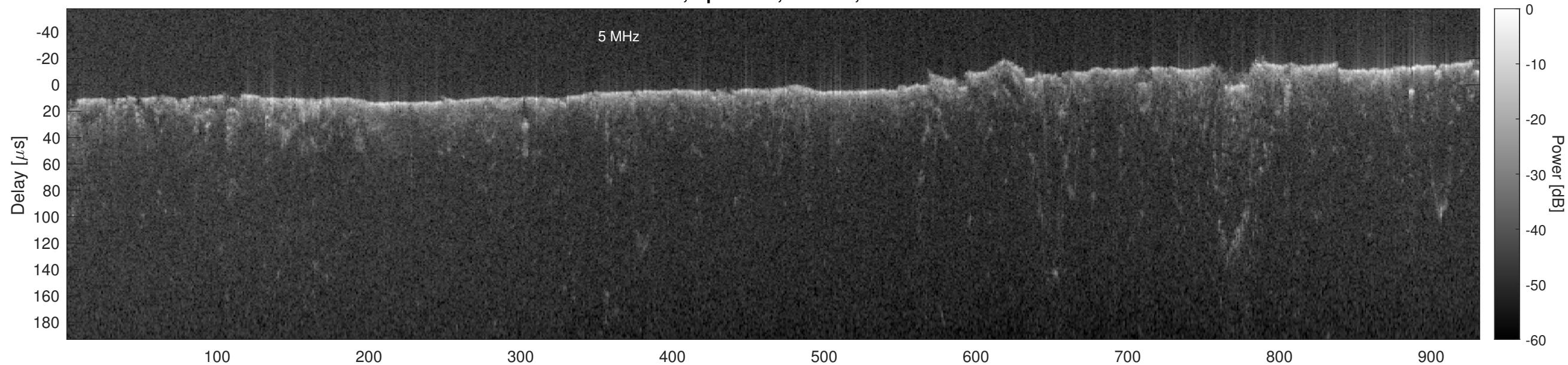
Orbit 5051, Optimized, Window, Channel 2
