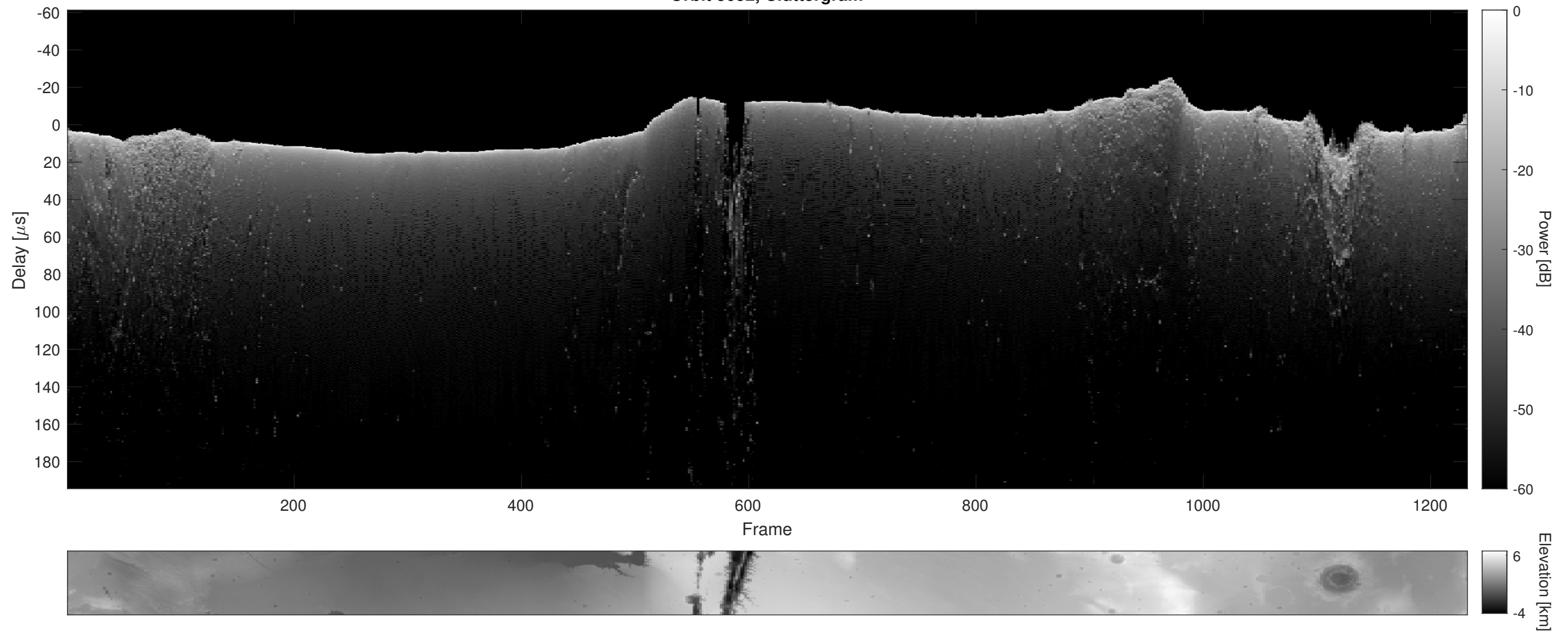
Orbit 5052, Cluttergram
