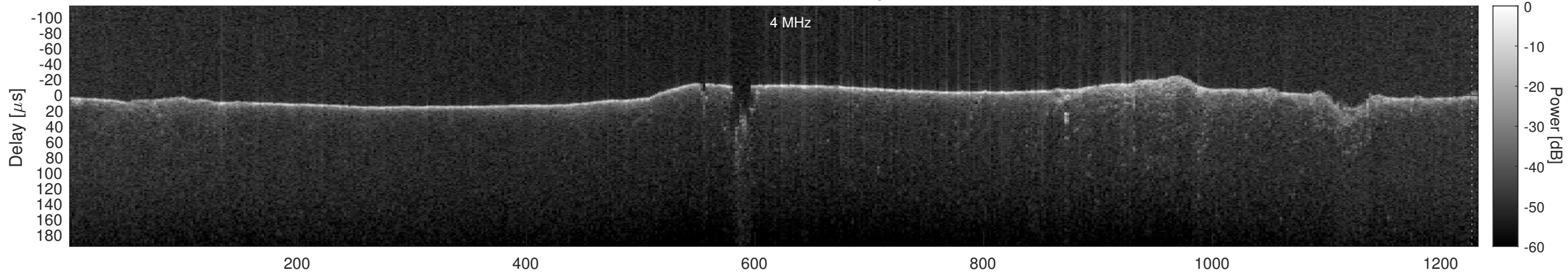
Orbit 5052, Cluttergram
