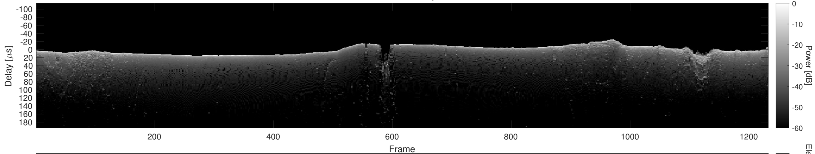
Orbit 5052, Cluttergram
