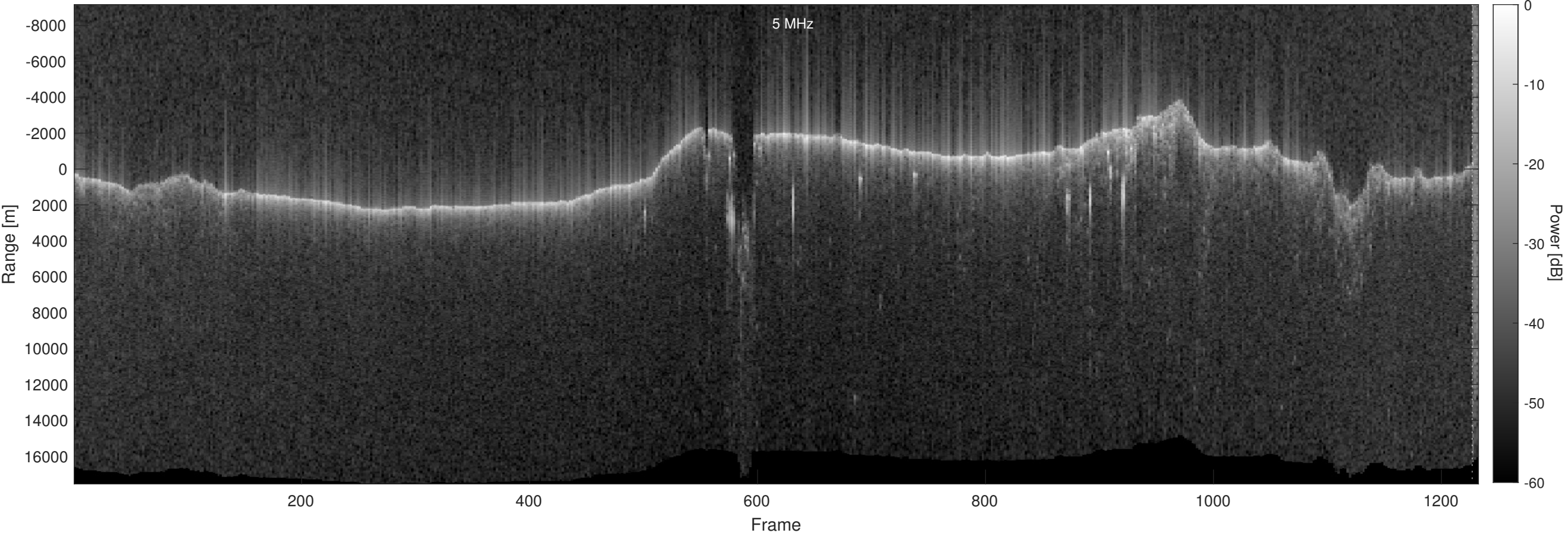
Orbit 5052, Optimized, No Window, Depth-Corrected, Channel 2
