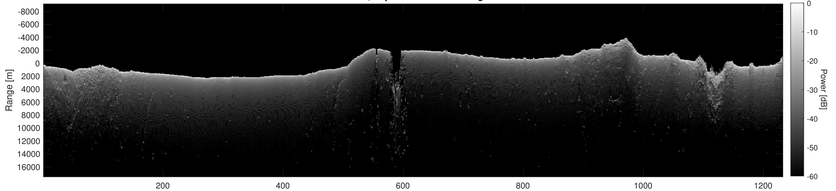
Orbit 5052, Depth-Corrected Cluttergram
