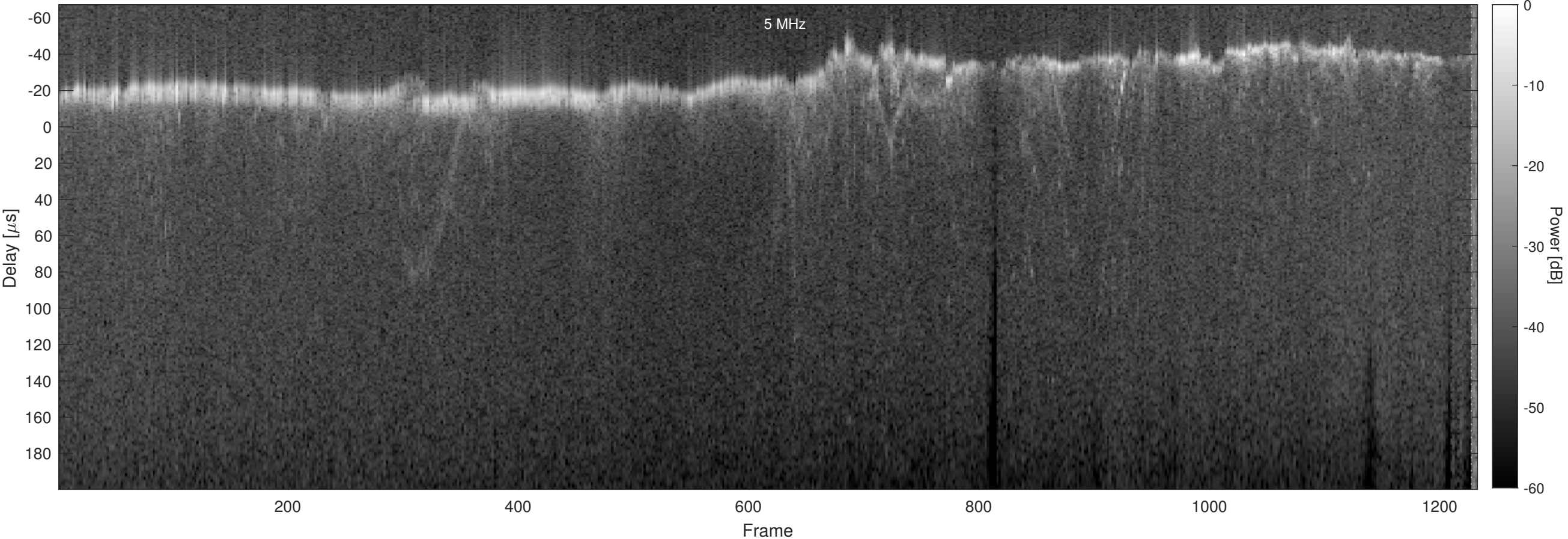
Orbit 5053, Chapman, Window, Channel 2
