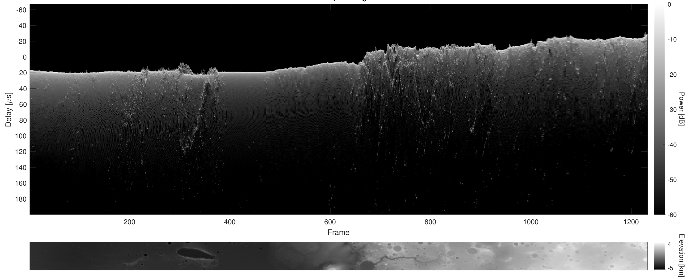
Orbit 5053, Cluttergram
