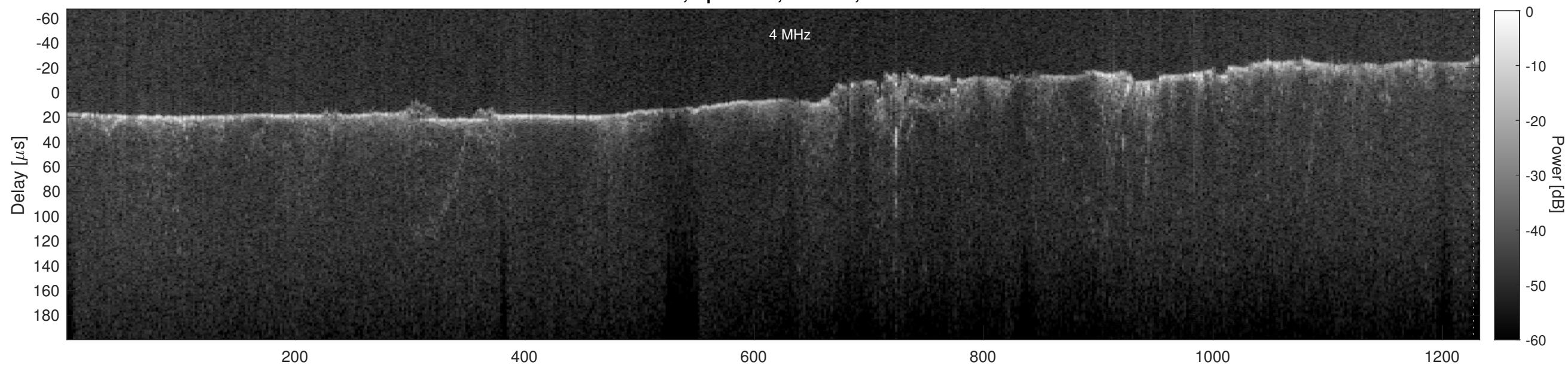
Orbit 5053, Cluttergram
