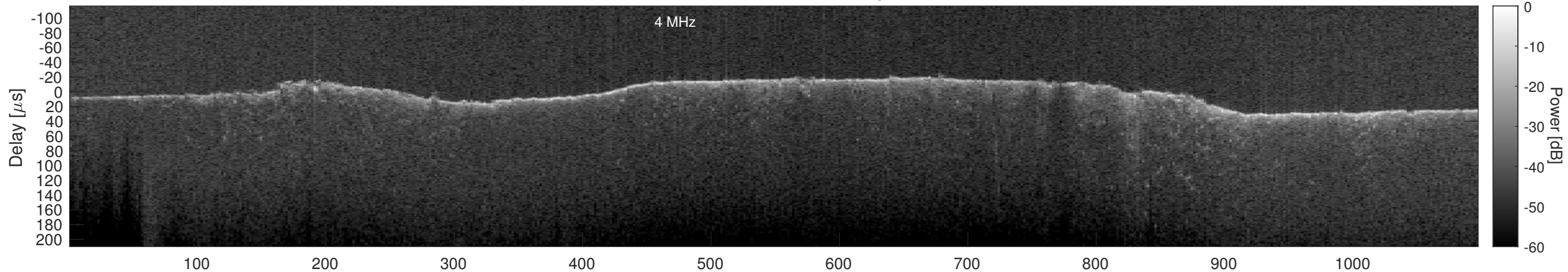
Orbit 5054, Cluttergram
