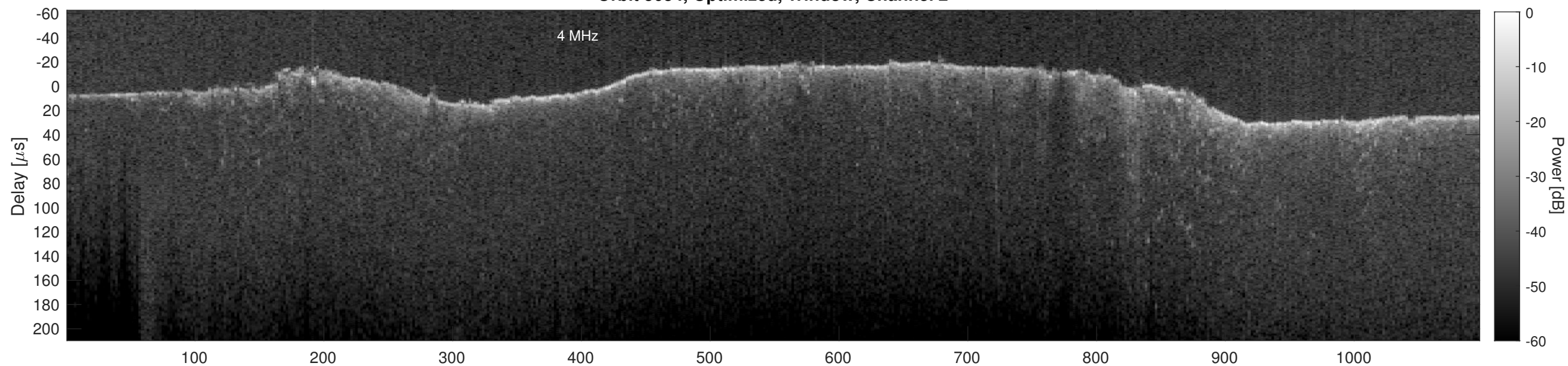
Orbit 5054, Cluttergram
