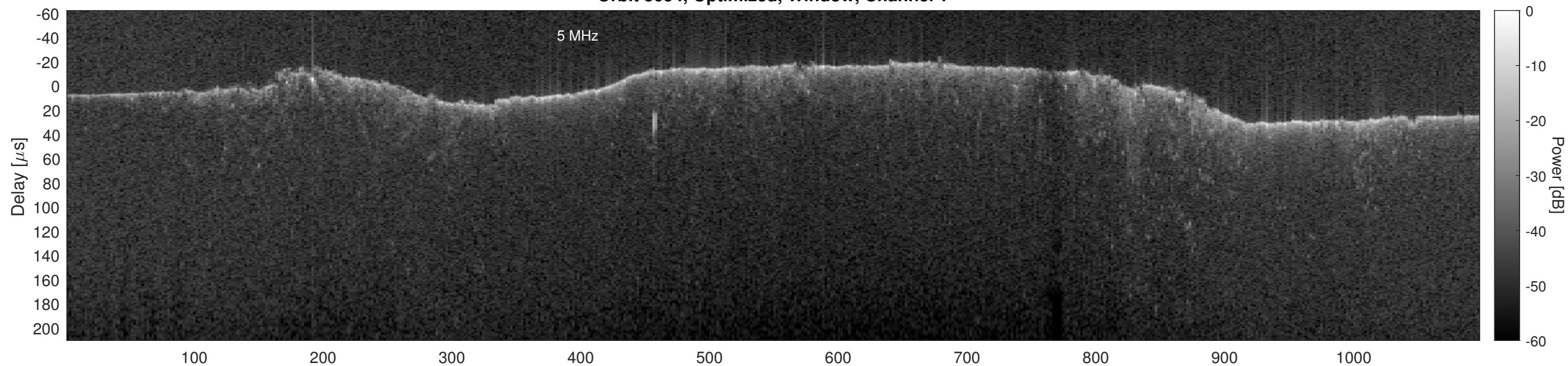
Orbit 5054, Optimized, Window, Channel 2
