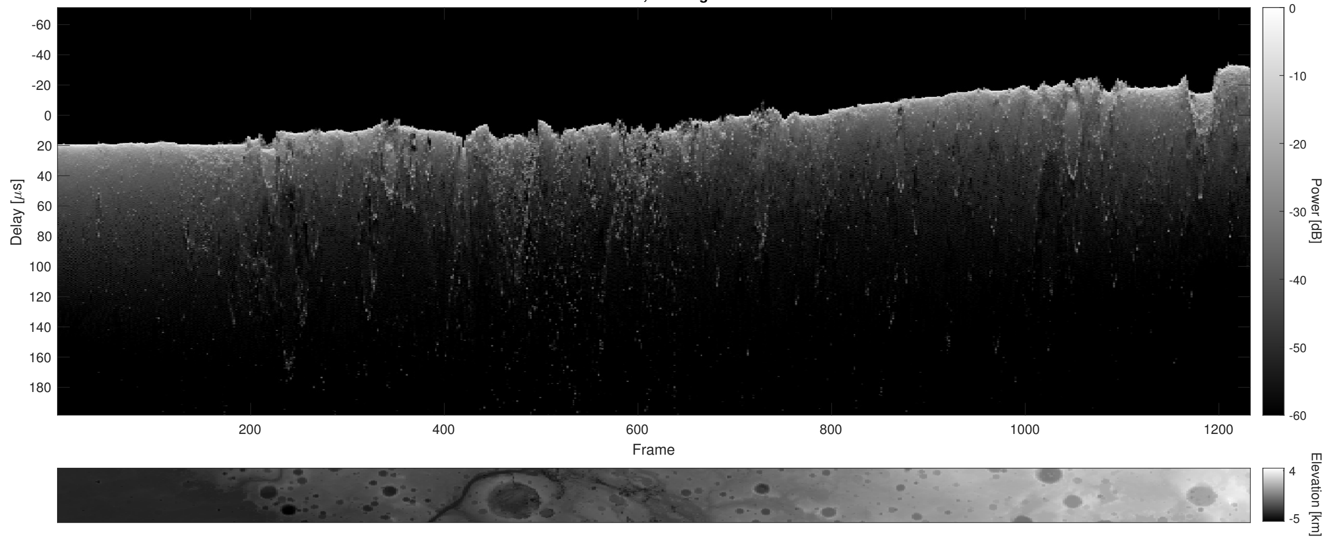
Orbit 5055, Cluttergram
