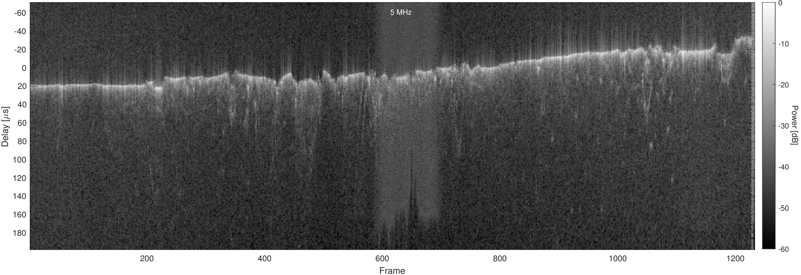
Orbit 5055, Optimized, No Window, Channel 2
