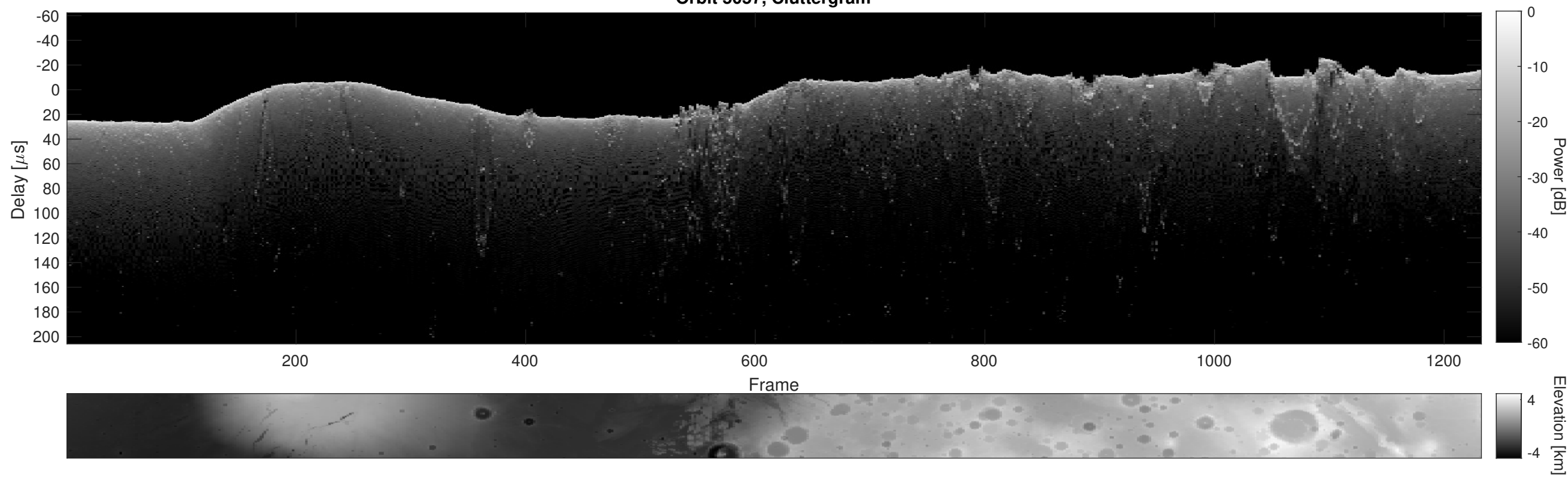
Orbit 5057, Cluttergram
