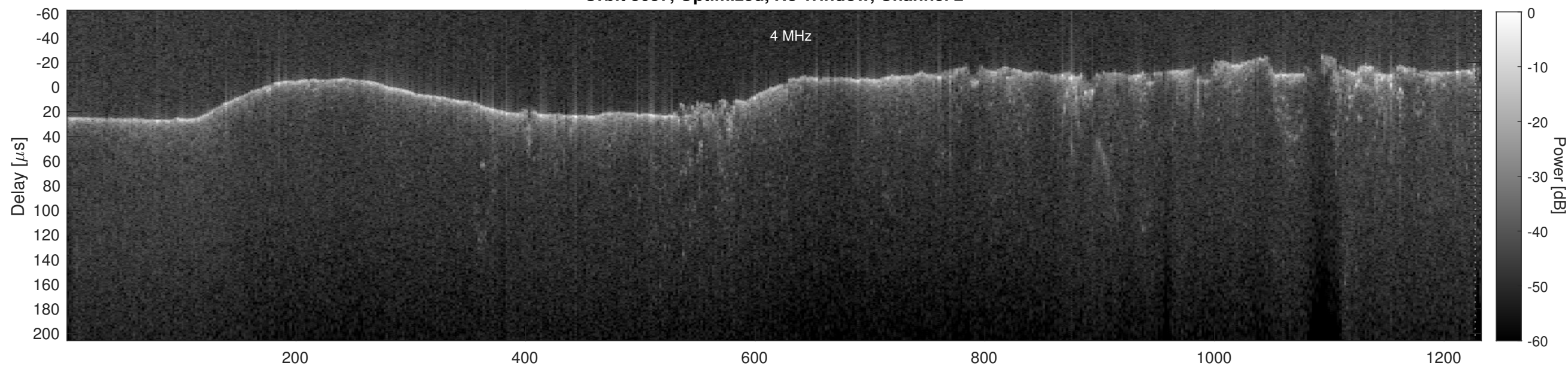
Orbit 5057, Cluttergram
