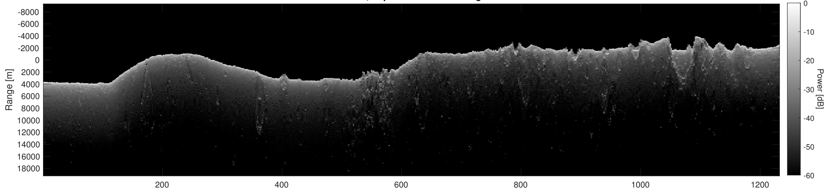
Orbit 5057, Depth-Corrected Cluttergram
