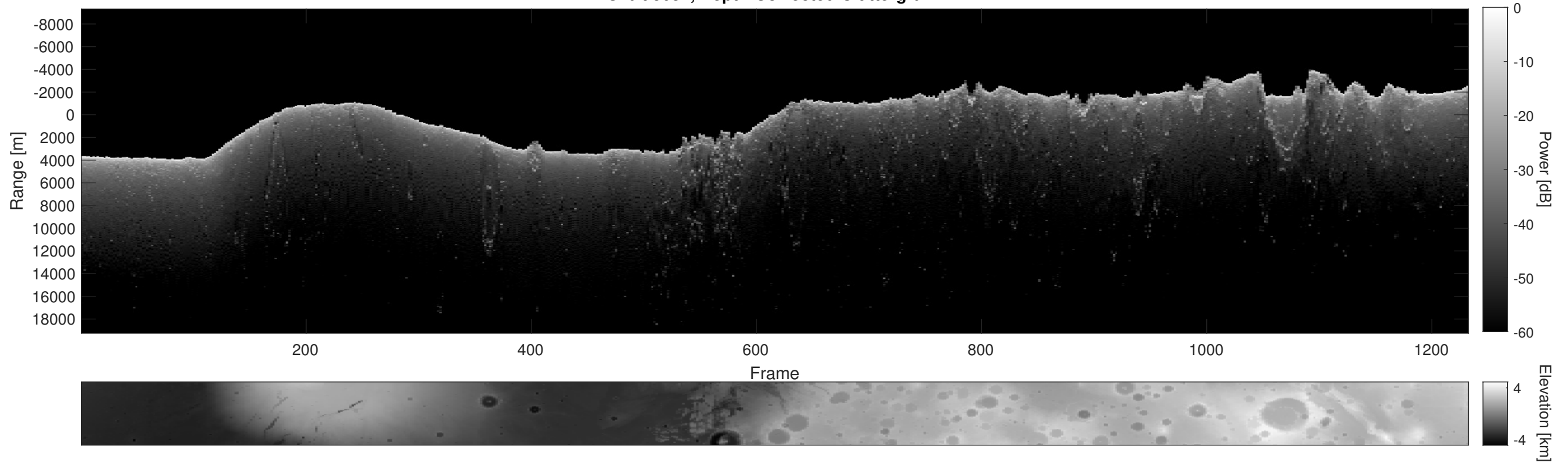
Orbit 5057, Depth-Corrected Cluttergram
