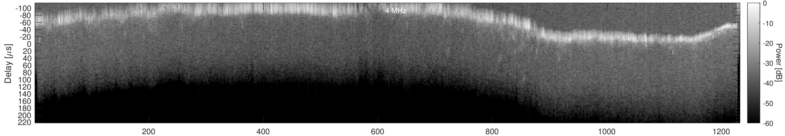
Orbit 5065, Window, Channel 2, Optimized
