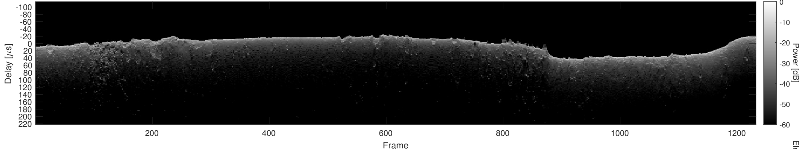
Orbit 5065, Cluttergram
