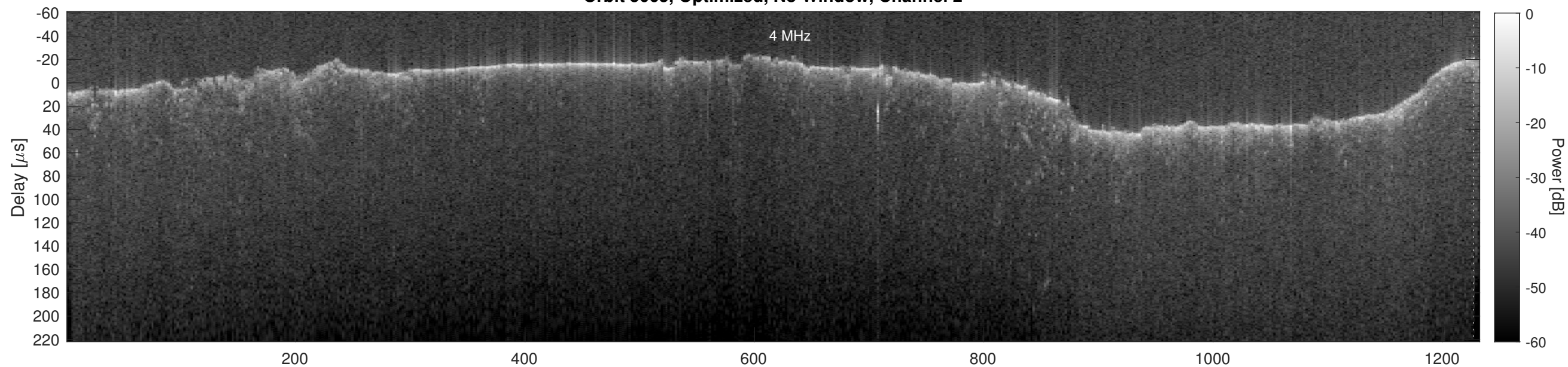
Orbit 5065, Cluttergram
