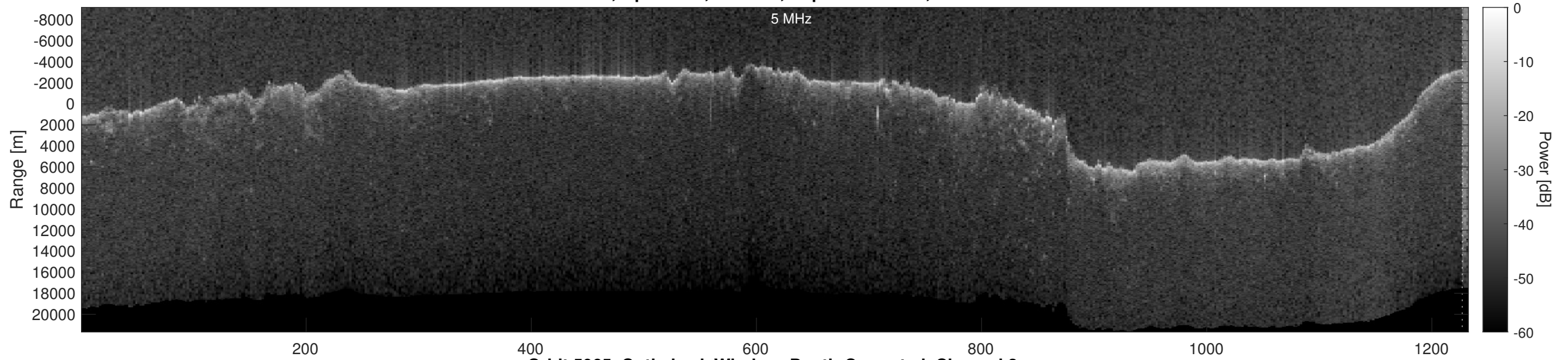
Orbit 5065, Optimized, Window, Depth-Corrected, Channel 2
