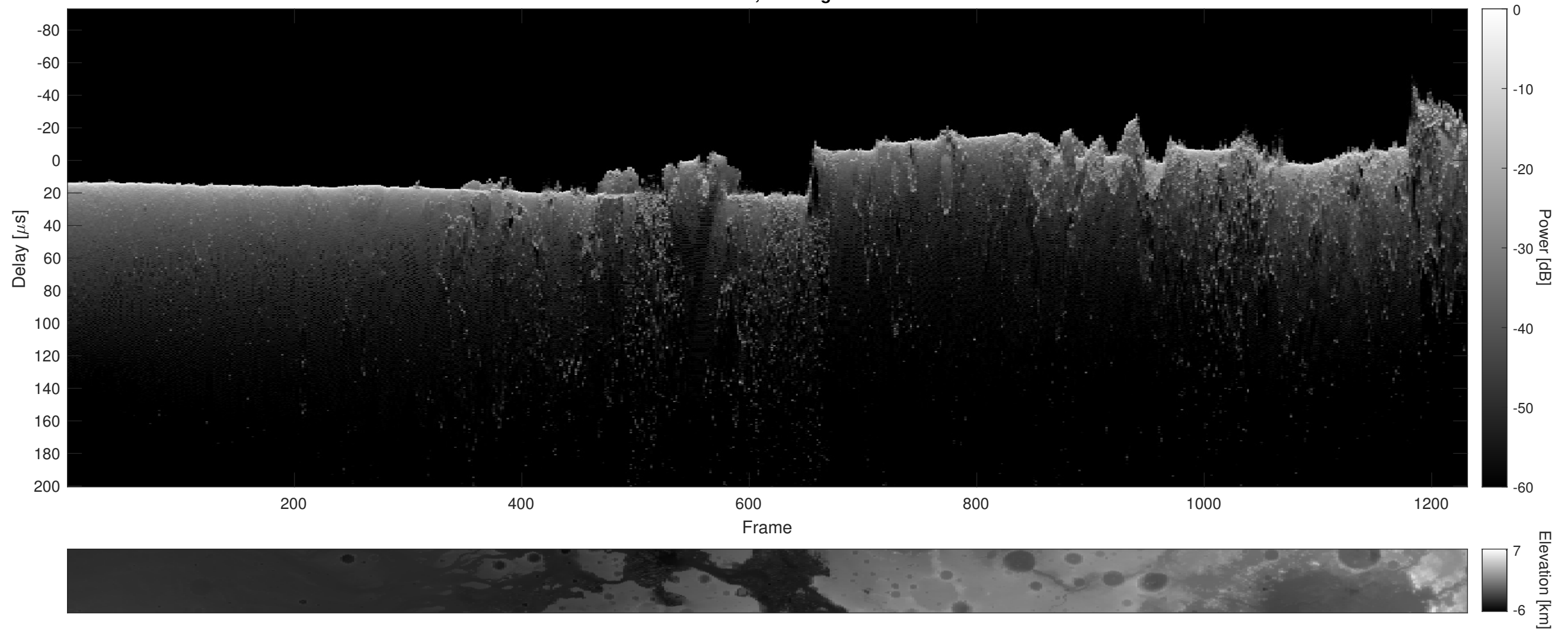
Orbit 5066, Cluttergram
