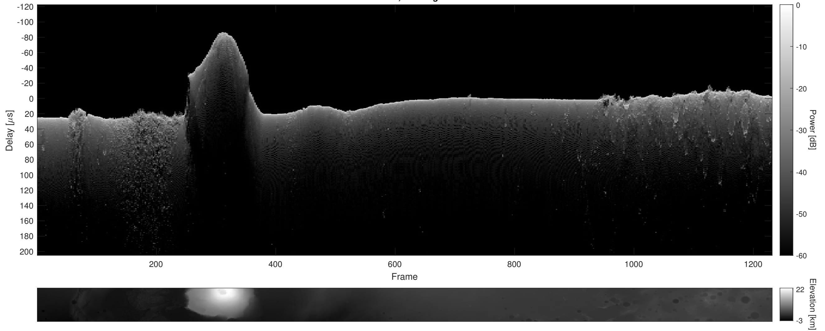
Orbit 5067, Cluttergram
