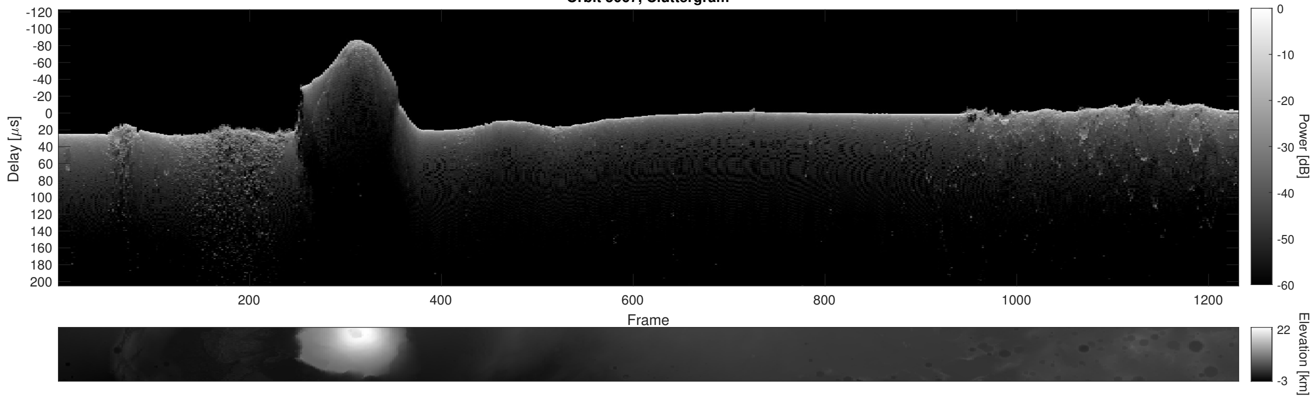
Orbit 5067, Cluttergram
