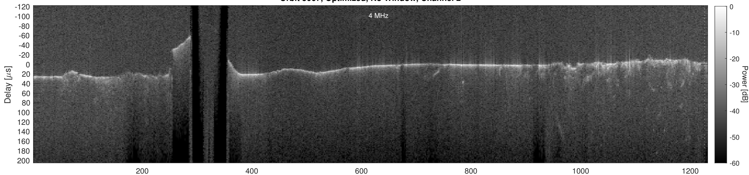
Orbit 5067, Cluttergram
