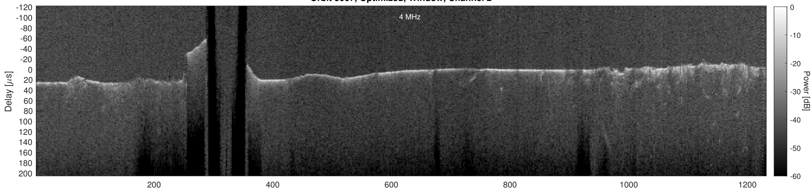
Orbit 5067, Cluttergram
