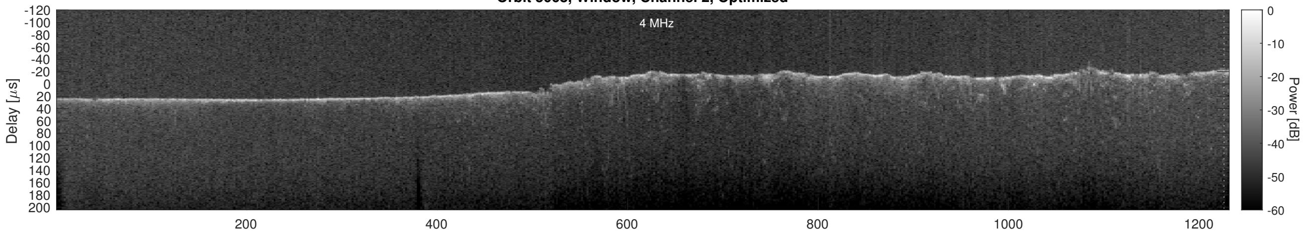
Orbit 5068, Cluttergram
