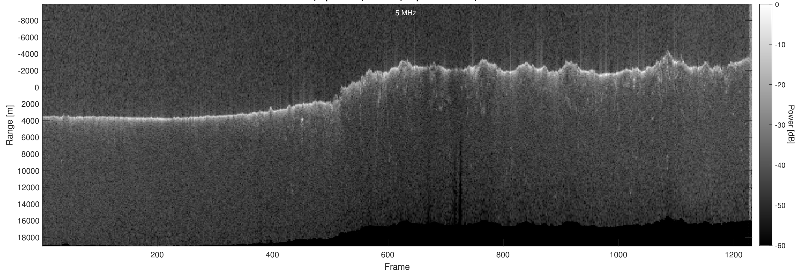
Orbit 5068, Optimized, Window, Depth-Corrected, Channel 2
