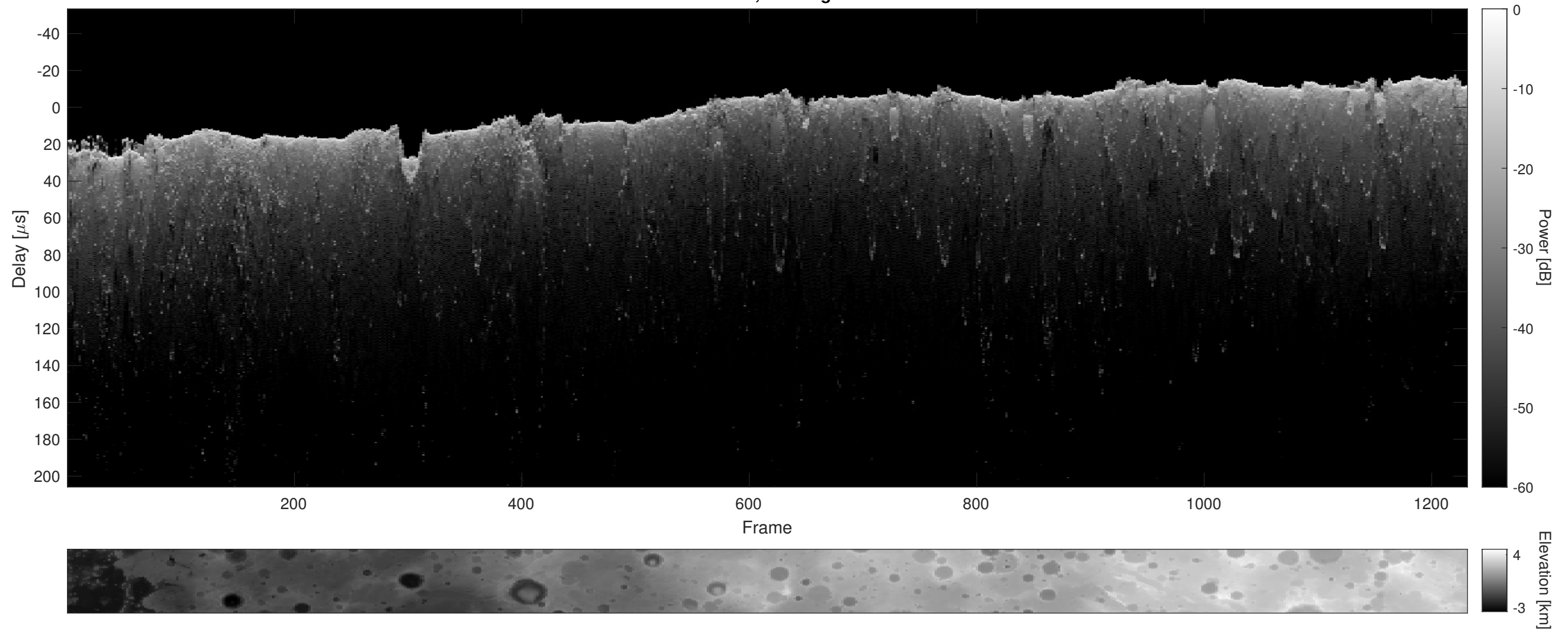
Orbit 5069, Cluttergram
