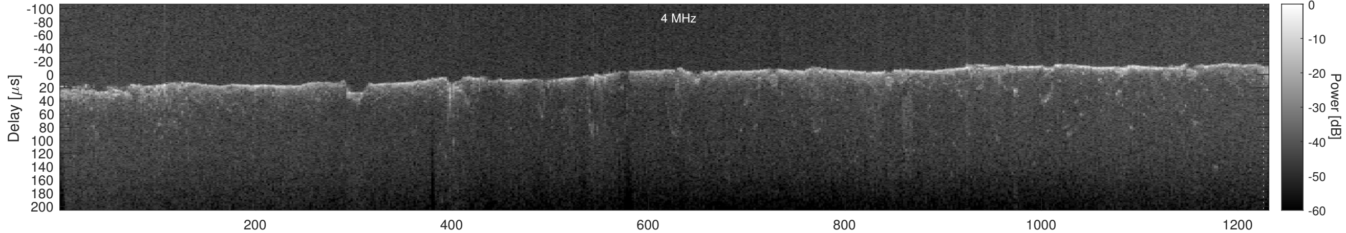
Orbit 5069, Cluttergram
