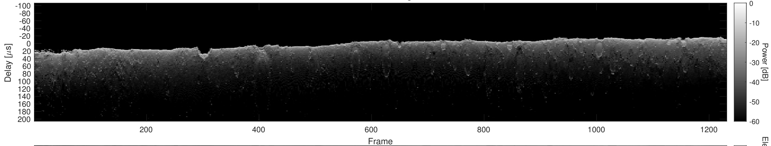
Orbit 5069, Cluttergram
