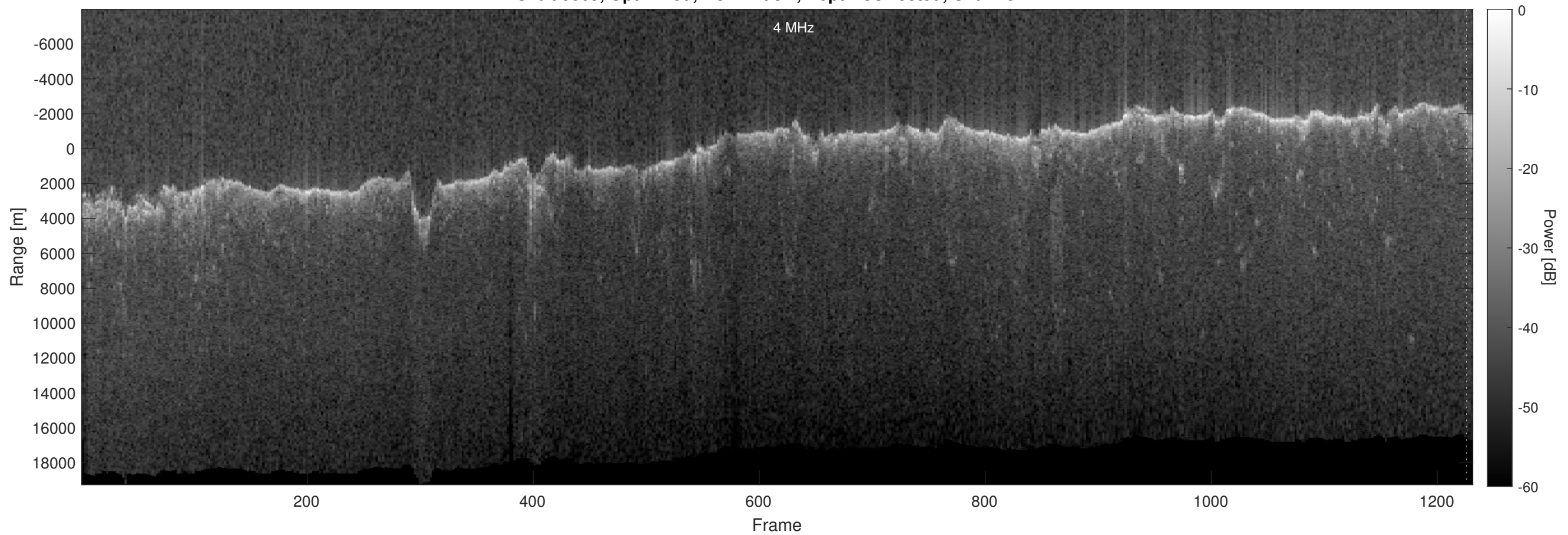
Orbit 5069, Optimized, No Window, Depth-Corrected, Channel 2
