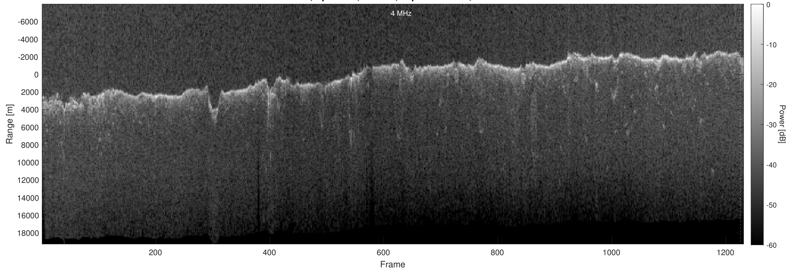
Orbit 5069, Optimized, Window, Depth-Corrected, Channel 2
