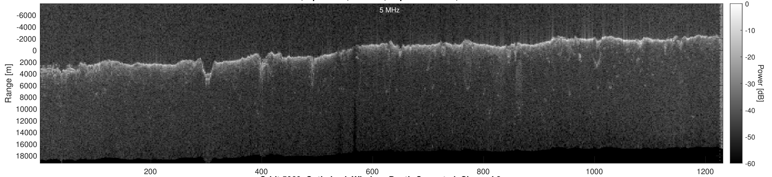
Orbit 5069, Optimized, Window, Depth-Corrected, Channel 2
