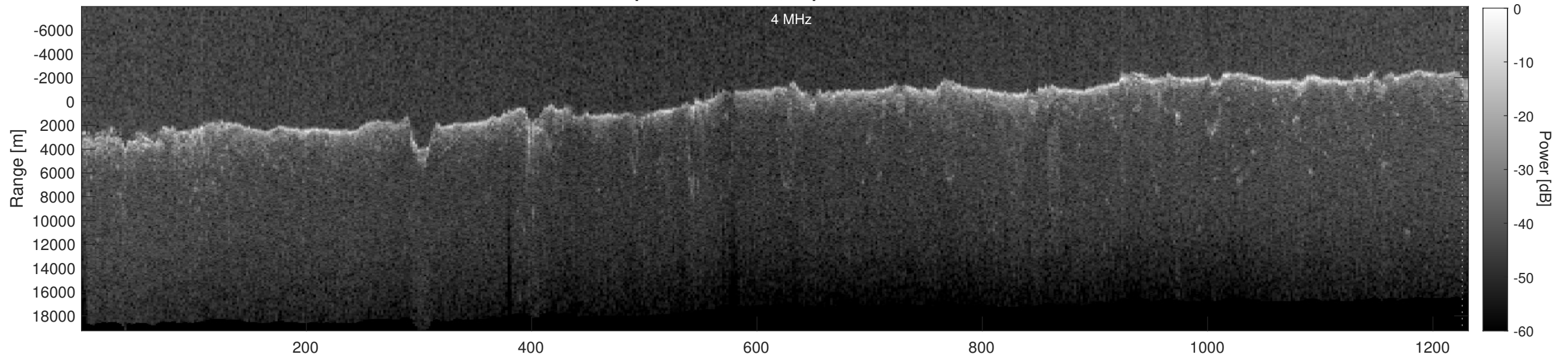
Orbit 5069, Depth-Corrected Cluttergram
