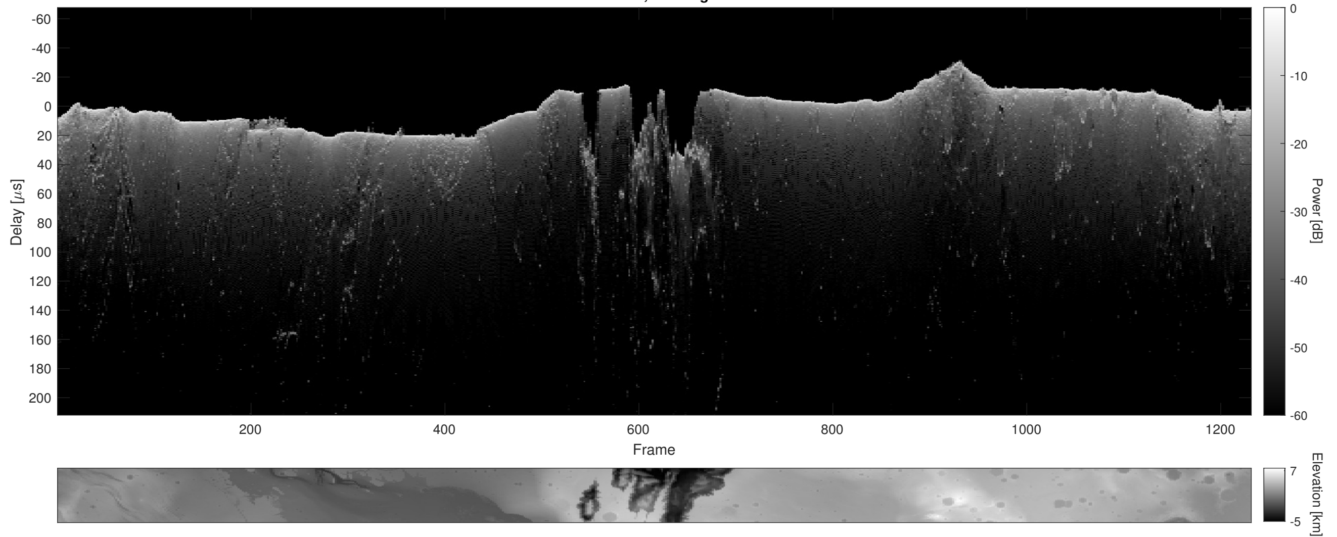
Orbit 5070, Cluttergram
