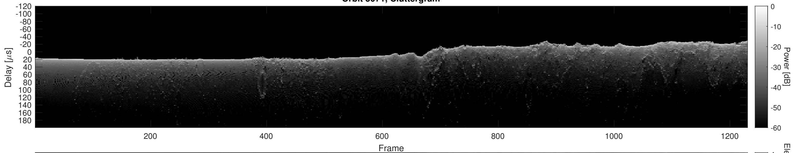
Orbit 5071, Cluttergram
