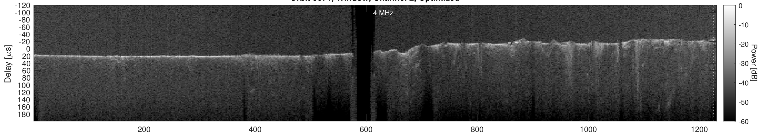
Orbit 5071, Cluttergram
