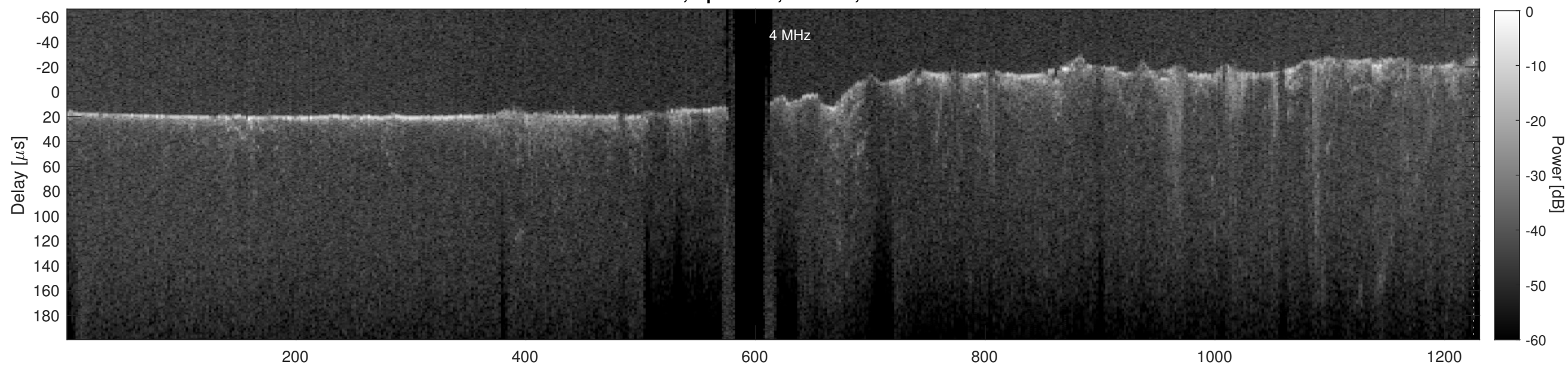
Orbit 5071, Cluttergram
