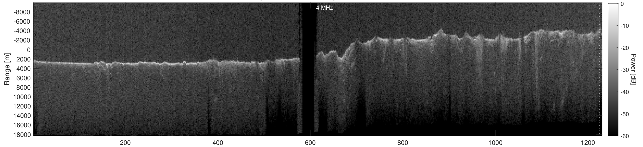
Orbit 5071, Depth-Corrected Cluttergram
