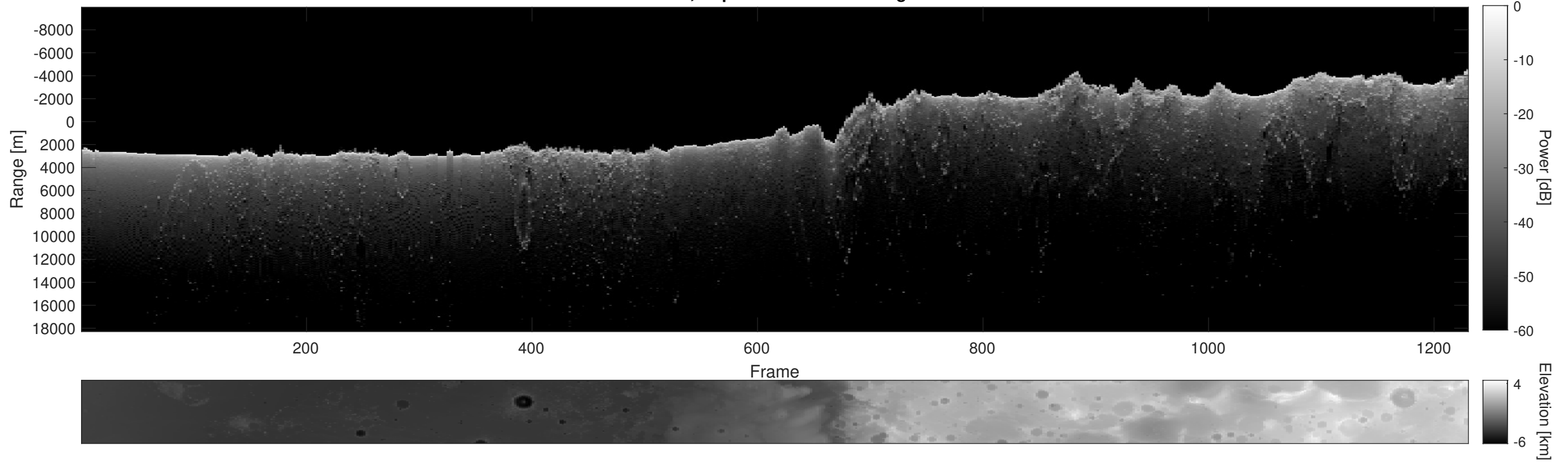
Orbit 5071, Depth-Corrected Cluttergram
