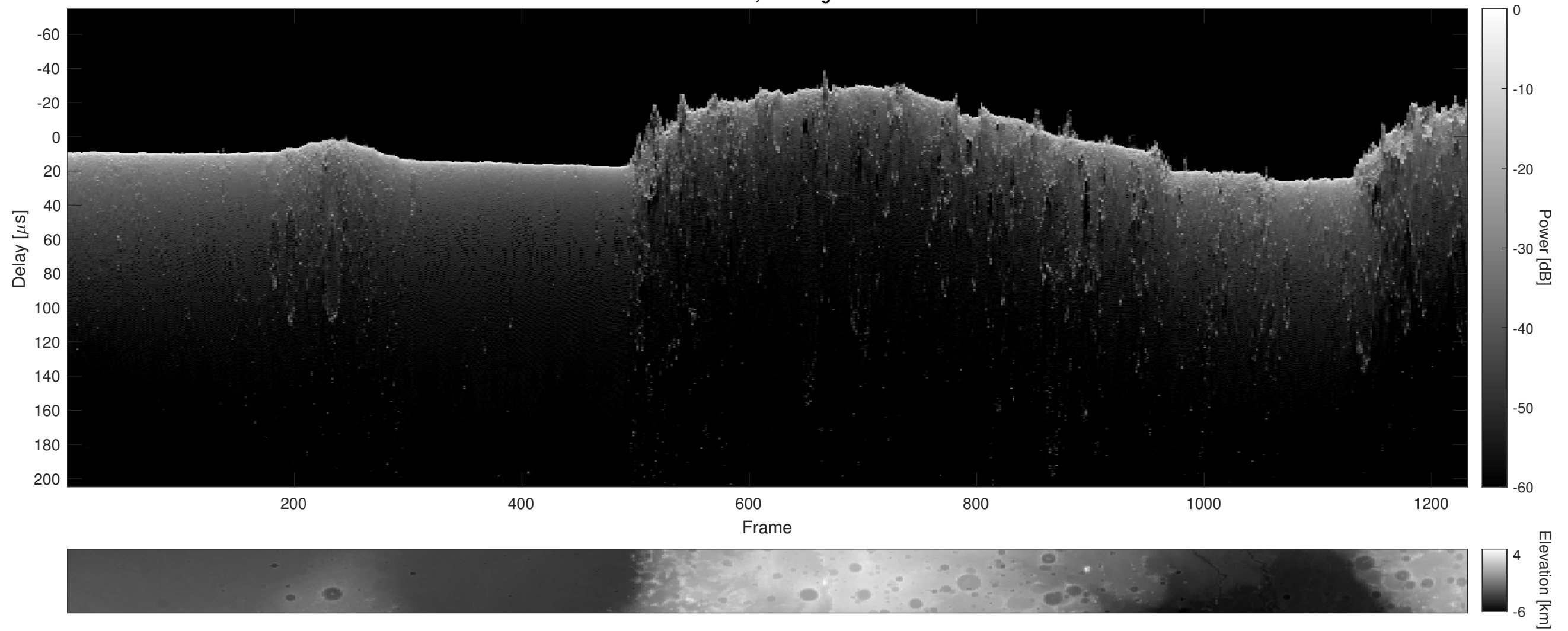
Orbit 5072, Cluttergram
