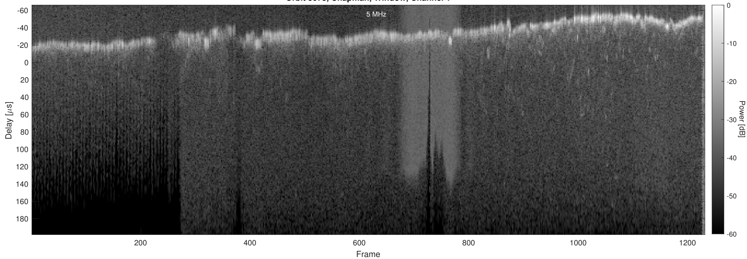
Orbit 5073, Chapman, Window, Channel 2
