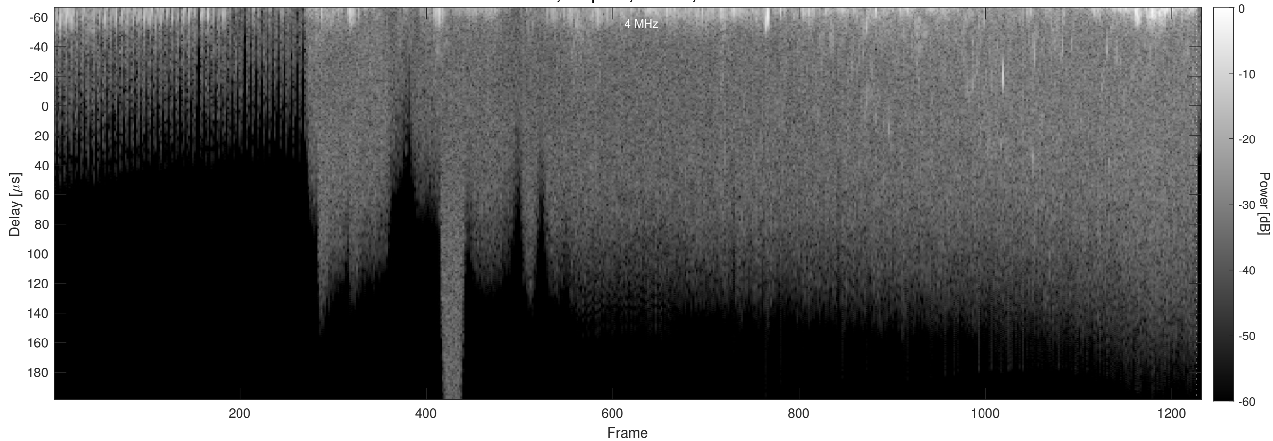
Orbit 5073, Chapman, Window, Channel 2
