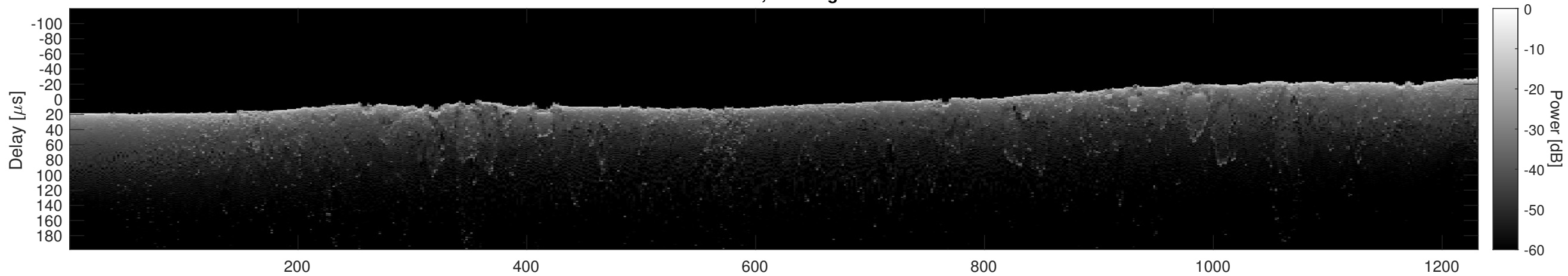
Orbit 5073, Cluttergram
