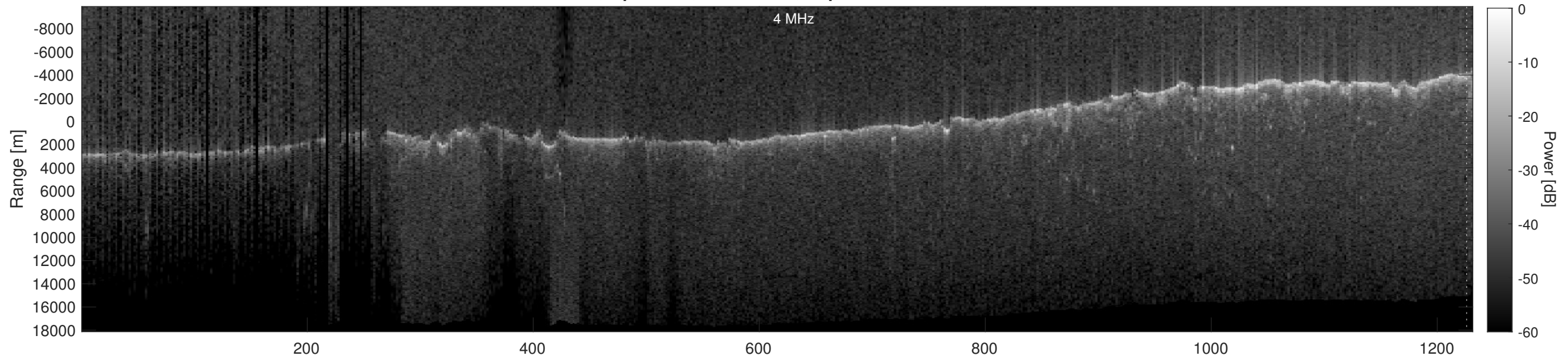
Orbit 5073, Depth-Corrected Cluttergram
