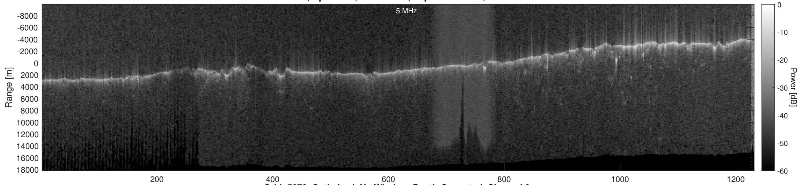
Orbit 5073, Optimized, No Window, Depth-Corrected, Channel 2
