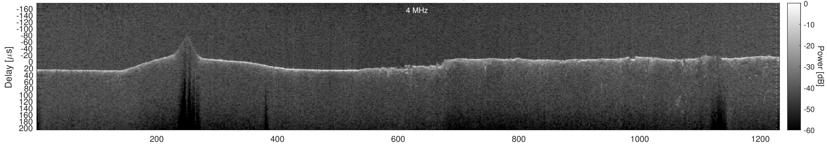
Orbit 5075, Cluttergram
