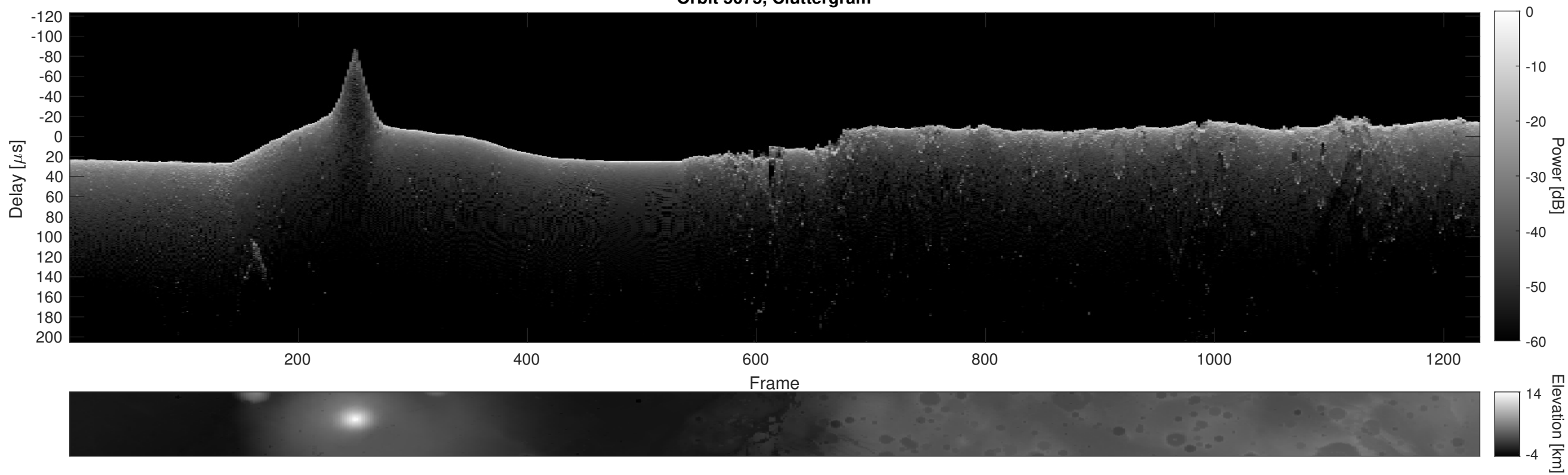
Orbit 5075, Cluttergram
