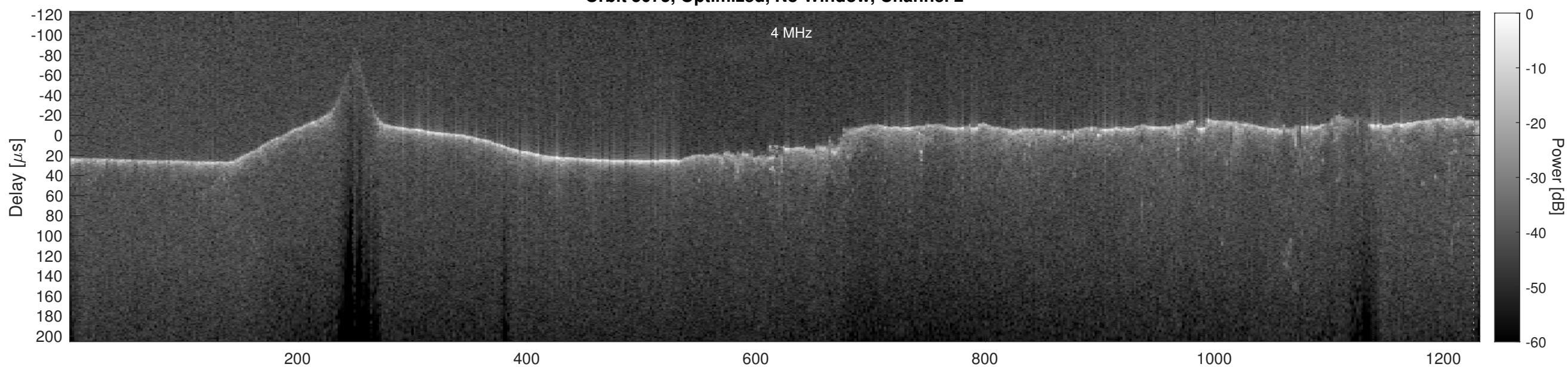
Orbit 5075, Cluttergram
