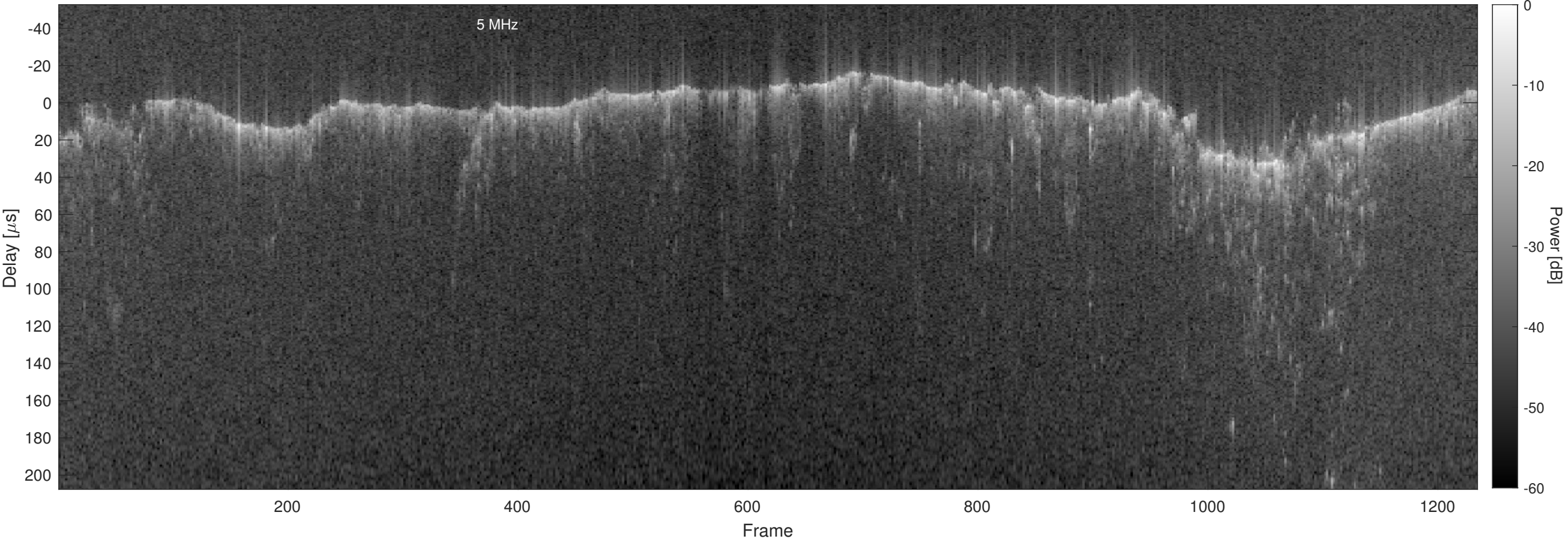
Orbit 5076, Optimized, No Window, Channel 2
