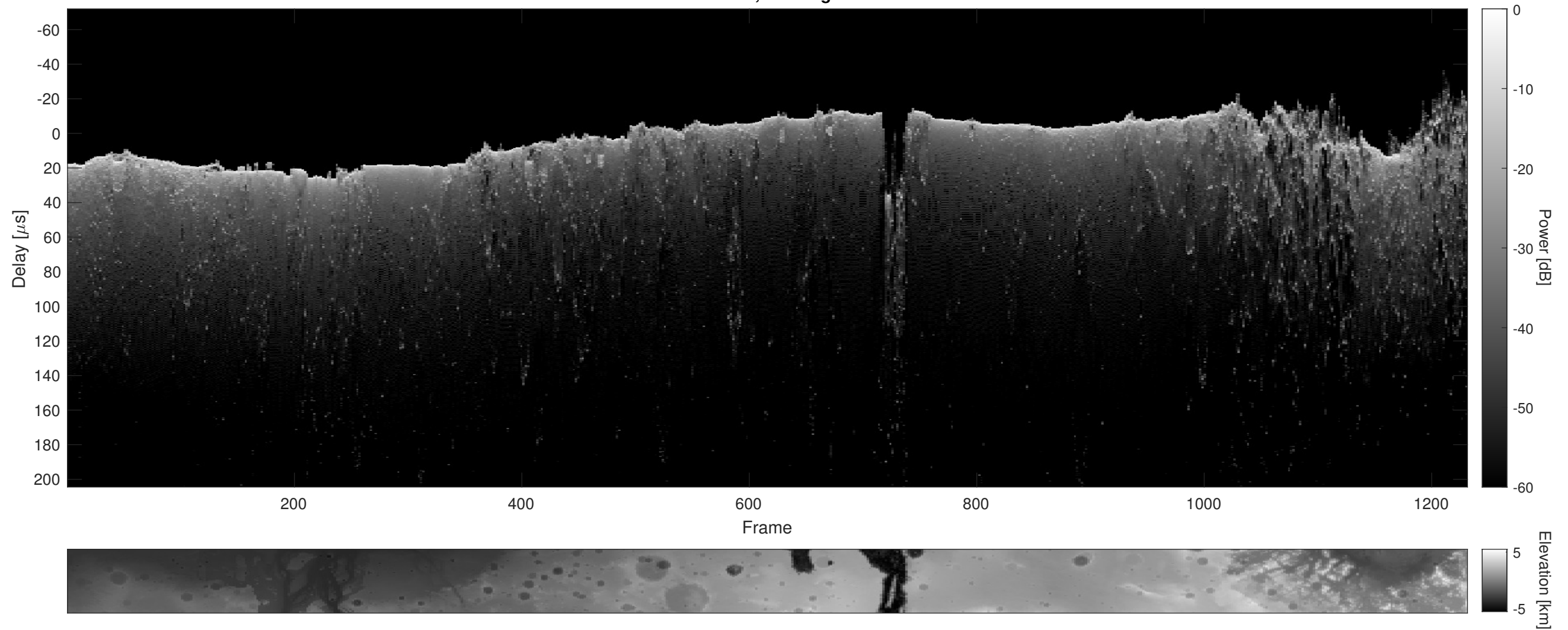
Orbit 5077, Cluttergram
