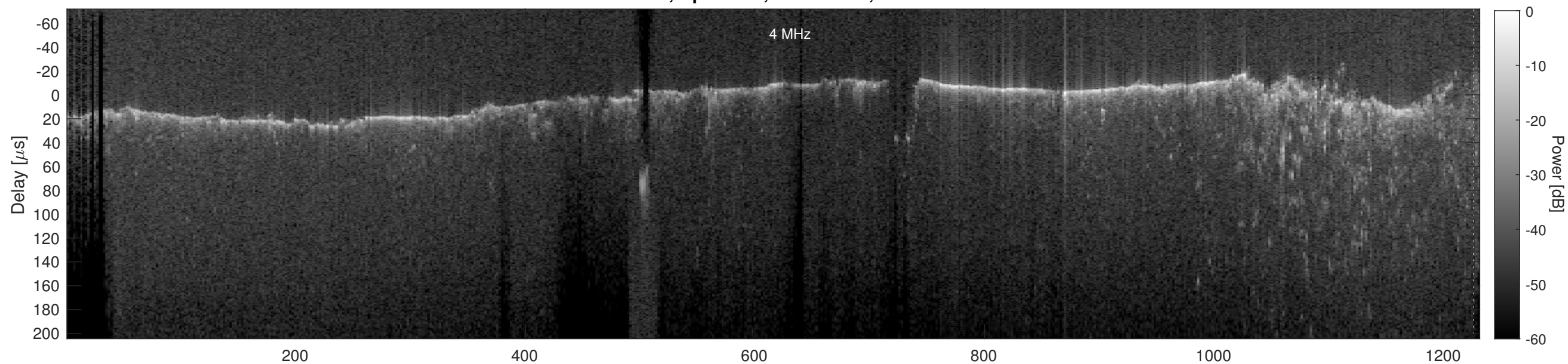
Orbit 5077, Cluttergram
