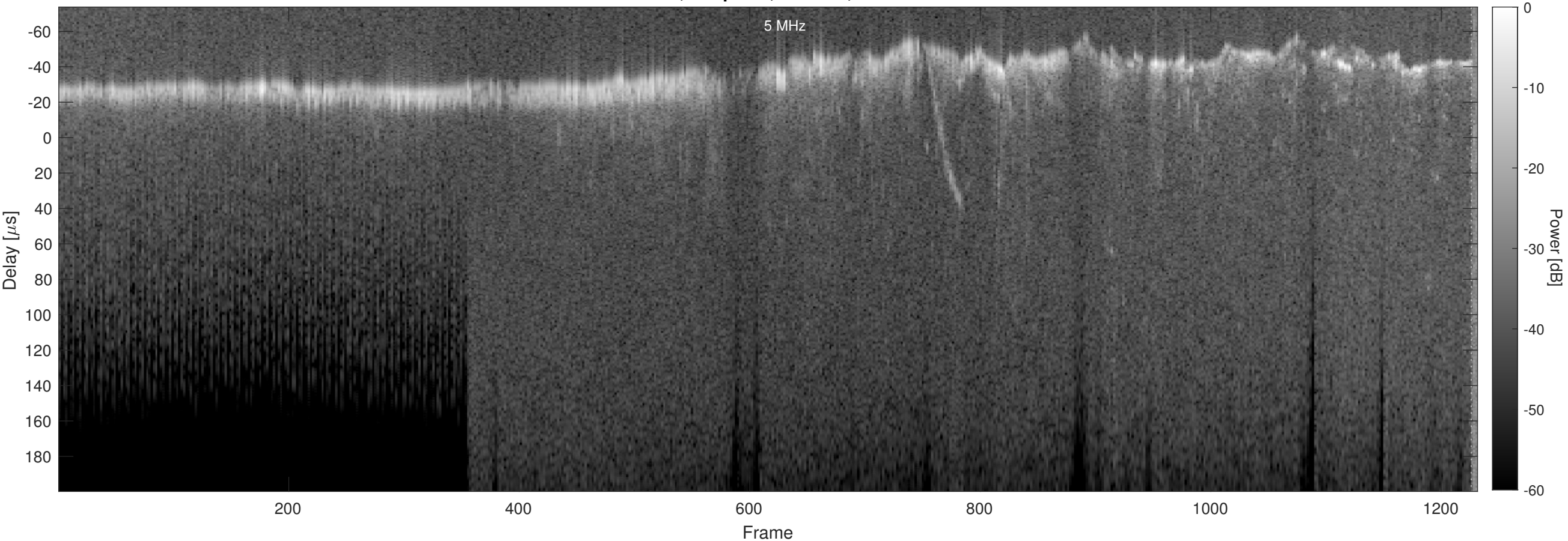
Orbit 5078, Chapman, Window, Channel 2
