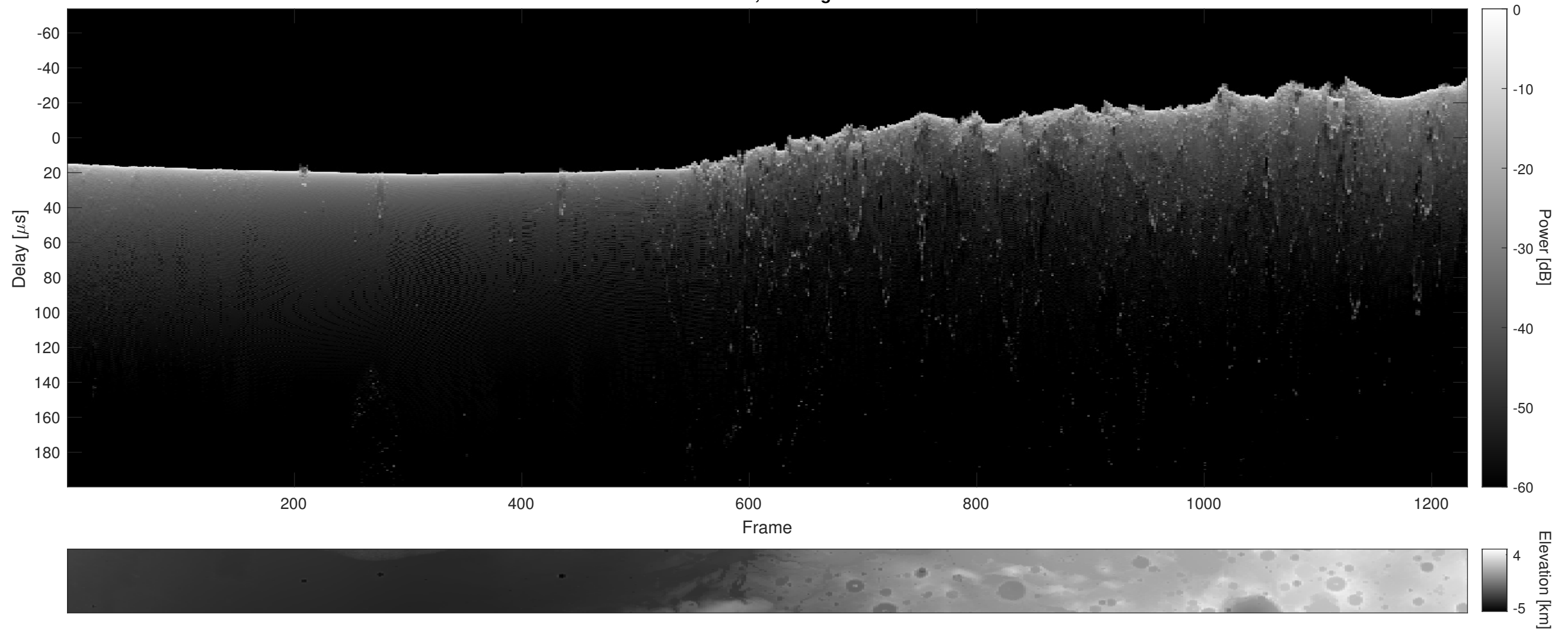
Orbit 5078, Cluttergram
