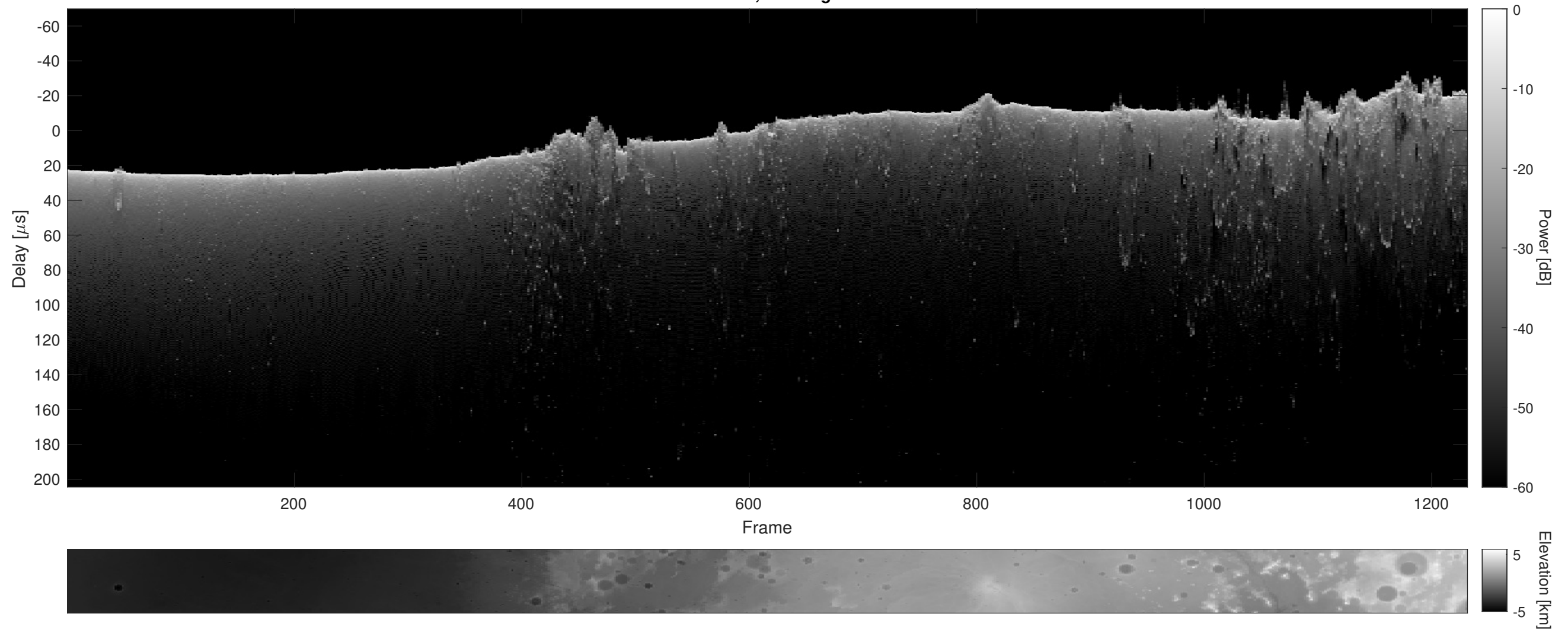
Orbit 5079, Cluttergram
