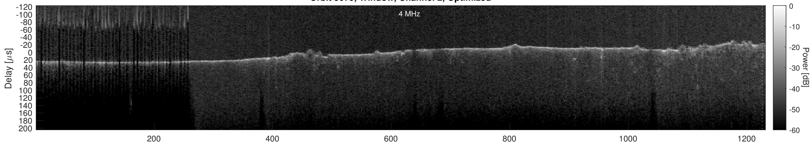
Orbit 5079, Cluttergram
