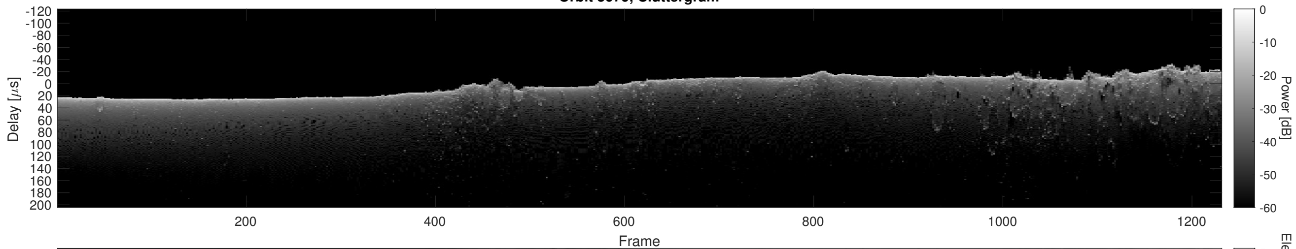
Orbit 5079, Cluttergram
