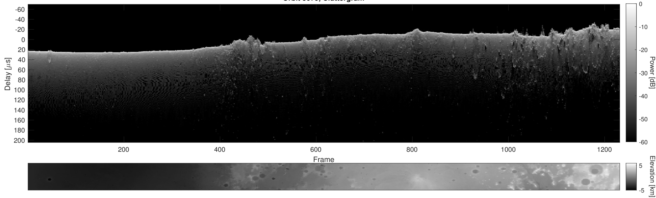
Orbit 5079, Cluttergram
