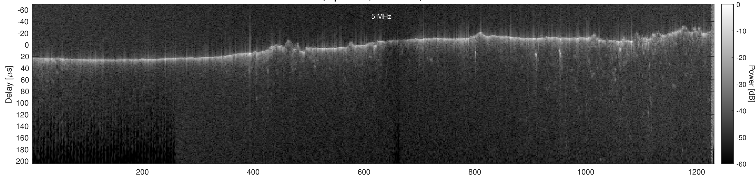
Orbit 5079, Optimized, No Window, Channel 2
