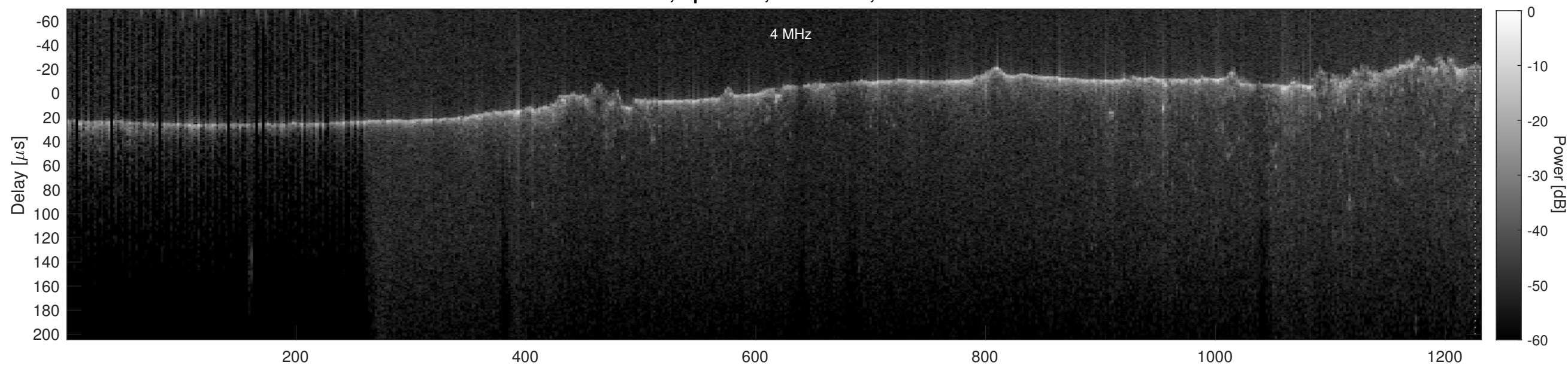
Orbit 5079, Cluttergram
