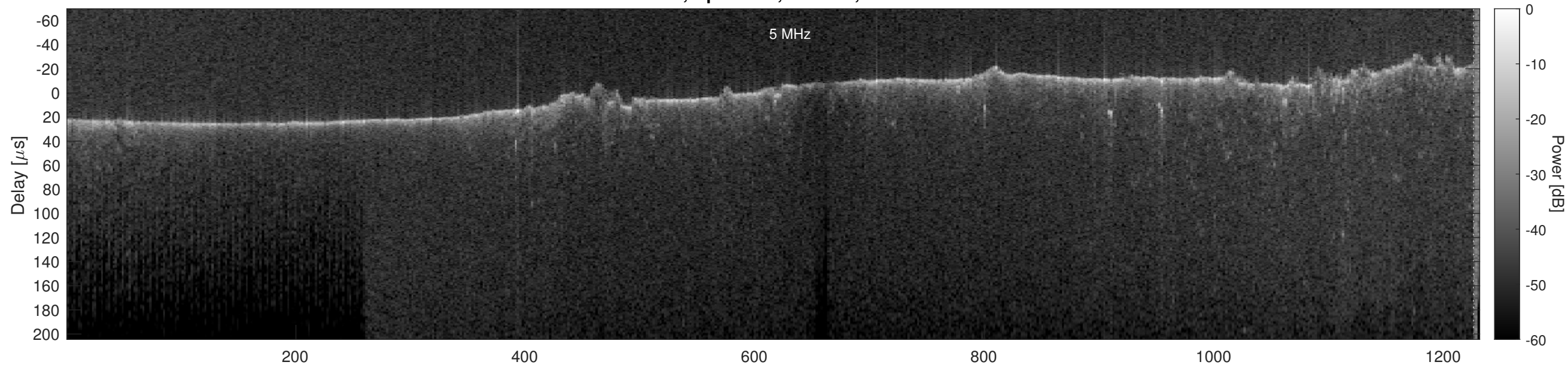
Orbit 5079, Optimized, Window, Channel 2
