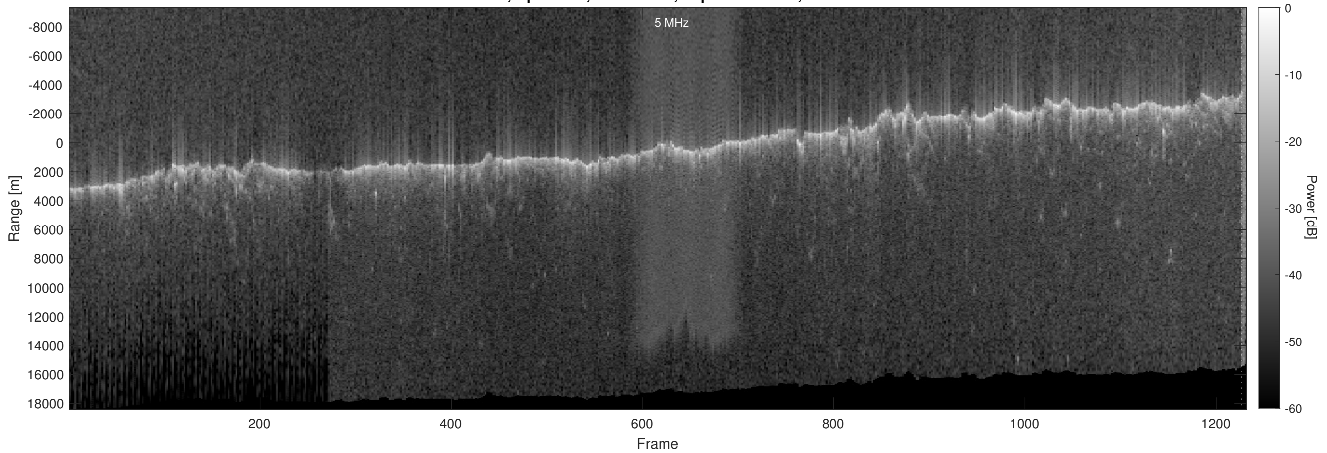
Orbit 5080, Optimized, No Window, Depth-Corrected, Channel 2
