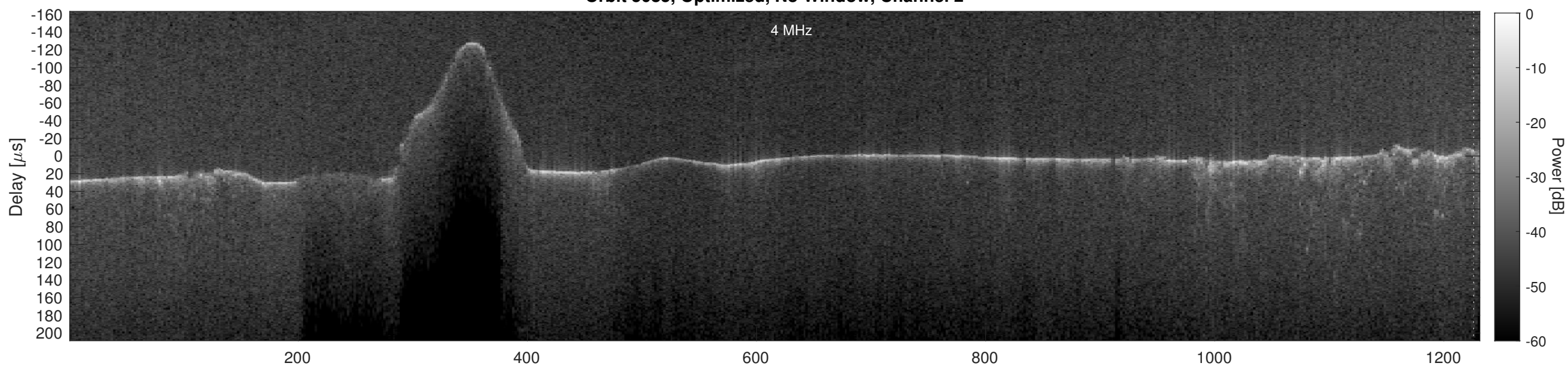
Orbit 5085, Cluttergram
