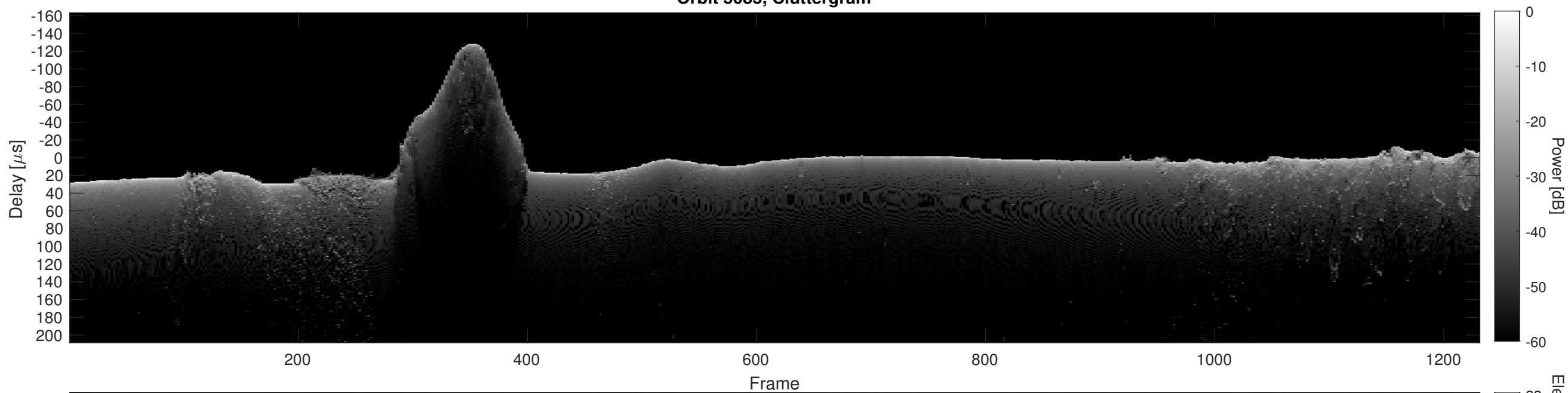
Orbit 5085, Cluttergram
